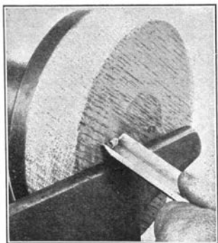
Fig. 271. Turning the Face with Roughing Gouge.
