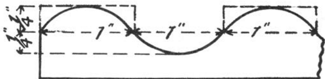
Fig. 51. One-inch Bead and Cove.
