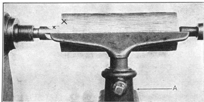
Fig. 9. Setting the Tee Rest.
