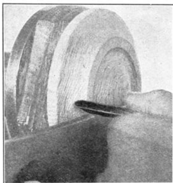
Fig. 128. Scraping with Round Nosed Tool.
