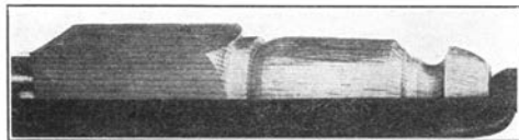
Fig. 250. Second Step in Turning Footstool Leg.
