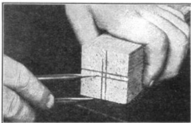
Fig. 3. Using the Compasses to Find the Center.
