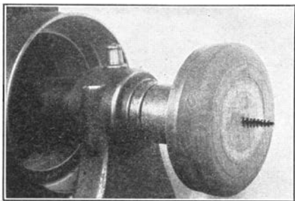
Fig. 268. Screw Chuck.
