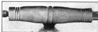
Fig. 69. End Beads Turned.
