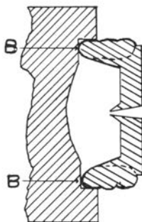
Fig. 168 Section of Napkin Ring in Cup Chuck.
