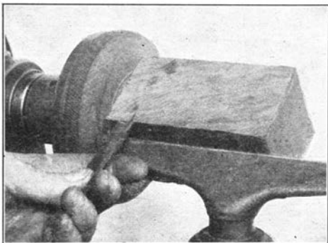
Fig. 100. Blank on Screw Chuck (See Fig. 113).
