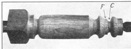
Fig. 95. Cavetto Turned.
