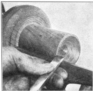
Fig. 107. Cutting Rebate.
