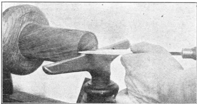
Fig. 104. Cutting Rebate.
