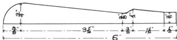
Fig. 133. Tool Handle.
