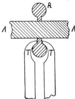
Fig. 295. Section Showing Cutting Position of Ring Tools.
