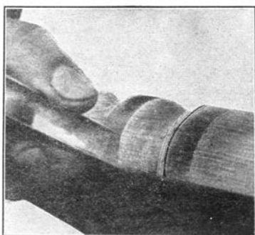
Fig. 42. Turning a Cove.
