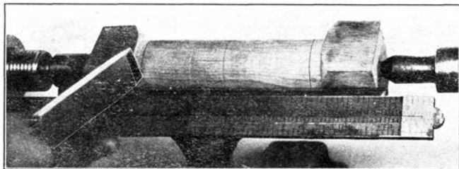
Fig. 75. Marking Spaces.
