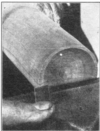
Fig. 105. Squaring End of Cover.
