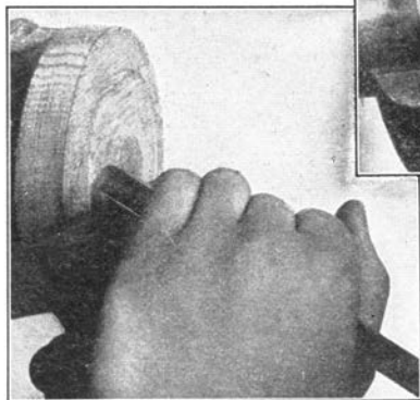
Fig. 126. Turning Face of Rosette.
