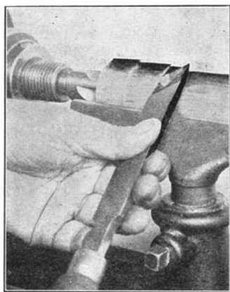
Fig. 21. Smoothing Up to a Shoulder.
