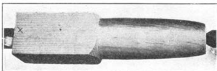
Fig. 249. First Step in Turning Footstool Leg.
