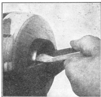
Fig. 171. Skew Chisel Smoothing Ring.
